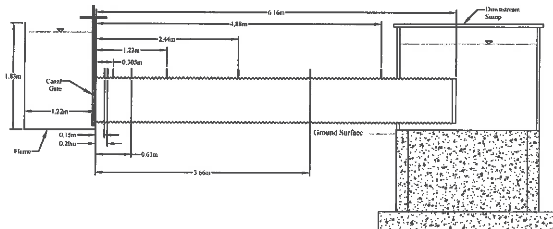
Figure 5. Side view of meter gate testing facility showing the pressure tap locations where measurements were taken.
